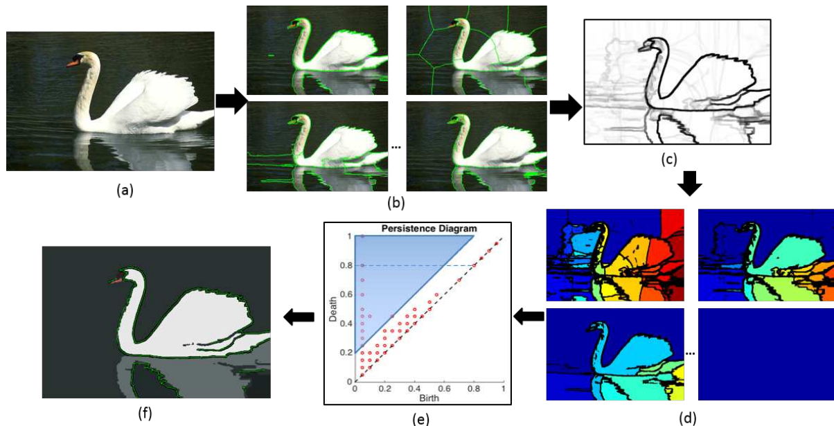
Figure 1. Pipeline of the proposed approach. (a) Original image. (b) Four samples from the segmentation set. The segmentation set generated by varying parameters of four algorithms are used as an input set. (c) A connectivity probability map is constructed. (d) A set of labeled images, which corresponds to the filtration set for the topological persistence analysis, is generated by thresholding the connectivity probability map. (e) Persistence diagram of the filtration shown in (d) where each point in the diagram corresponds to a connected component in the filtration. (f) Segmentation result obtained by applying two thresholds in the persistence diagram.
